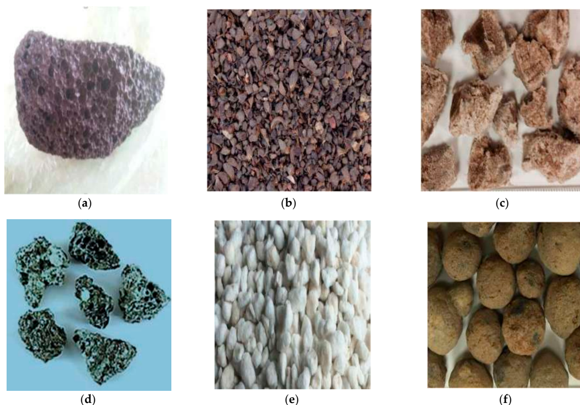
Figure 3. Different light weight aggregates (a) Pumice “Reprinted from ref. [57].” (b) Oil palm shell “Reprinted from ref. [71].” (c) Synthetic aggregate “Reprinted with permission from ref. [72]. Copyright 2018 Elsevier” (d) Oil palm shell (Boiler clinker) “Reprinted with permission from ref. [73]. Copyright 2016 Elsevier” (e) Expanded perlite “Reprinted from ref. [74].” (f) Lytag aggregate “Reprinted with permission from ref. [72]. Copyright 2018 Elsevier”.
