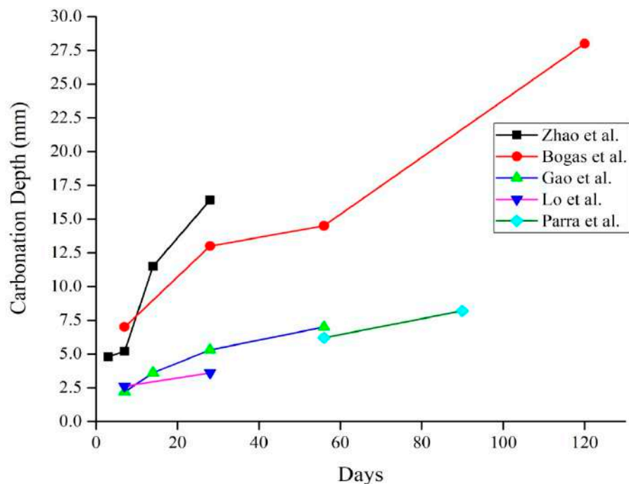
Figure 12. Carbonation depth of lightweight concrete [18,21,22,113,114].
