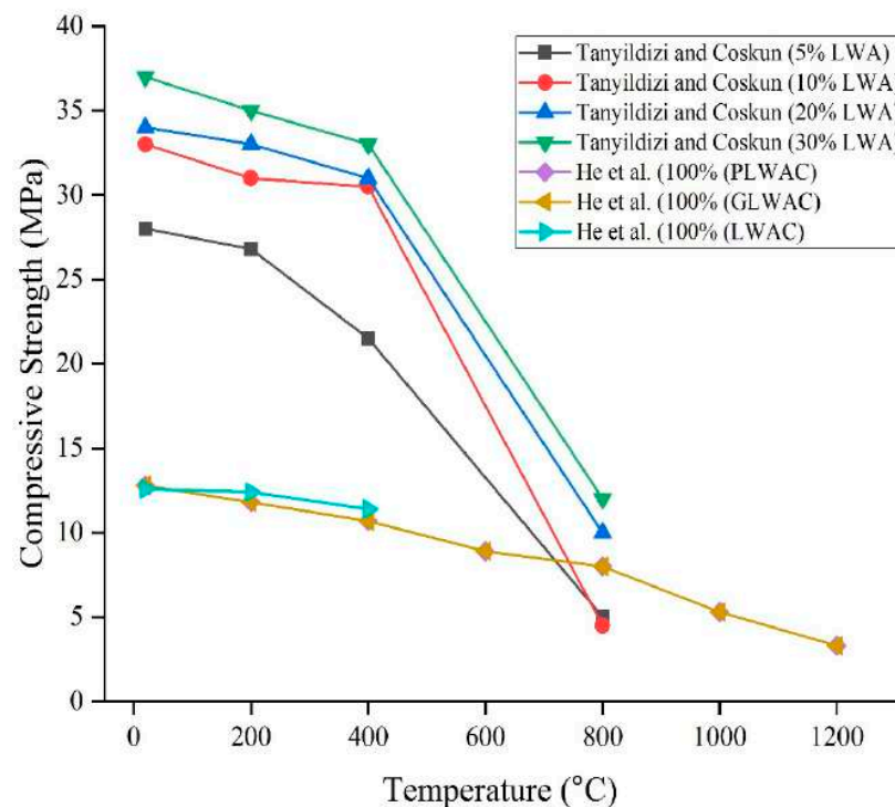
Figure 15. Compressive strength at high temperature [38,117].
