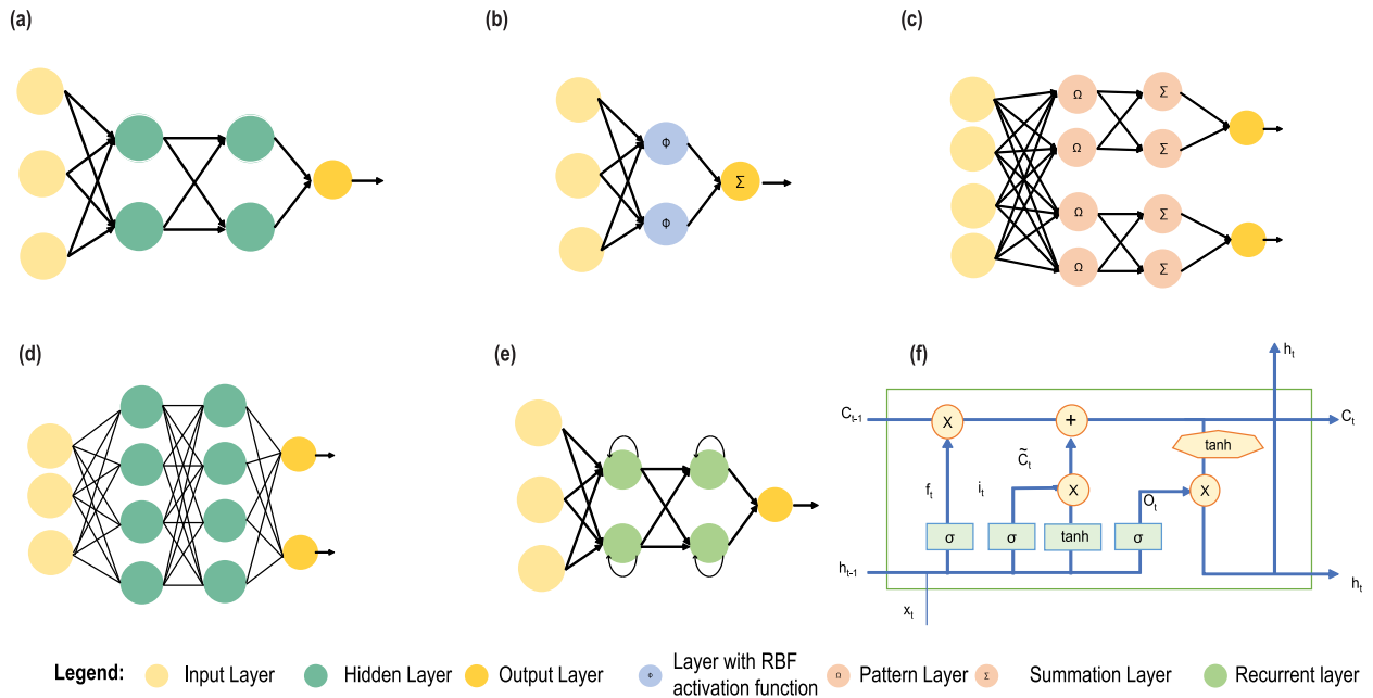
FIGURE 7. (a) An ANN architecture consisting of two hidden layers. In the input layer, there are three nodes, and there are two nodes for each hidden layer. In each node, an activation function takes the input from the previous layer. (b) An RBFNN architecture. The nodes denoted by \phi implements radial functions. (c) A PNN architecture. The pattern layer is denoted by \Omega , and the summation layer is denoted by \Sigma . This algorithm uses a probability distribution function. (d) DNN architecture. This network consists of four hidden layers which are fully connected. (e) RNN architecture. There are two recurrent layers which has some feedback connection. These connections help finding historical patterns in data. (f) LSTM cell structure. It uses some parameters which are, h_t (output value of a cell), x_t (input value of a cell), f_t (forget gate value), i_t (input gate value), O_t (output gate value), C_t (cell state), \tilde{C}_t (candidate value). \sigma , and \tanh are the activation functions. The output h_t is calculated as h_t = \tanh(c_t) \times O_t , where C_t = f_t C_{t-1} + i_t \tilde{C}_t .
