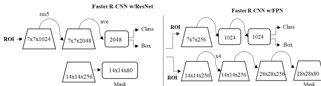
Figure 3. Mask-region based Convolutional Neural Network (Mask R-CNN) framework.
