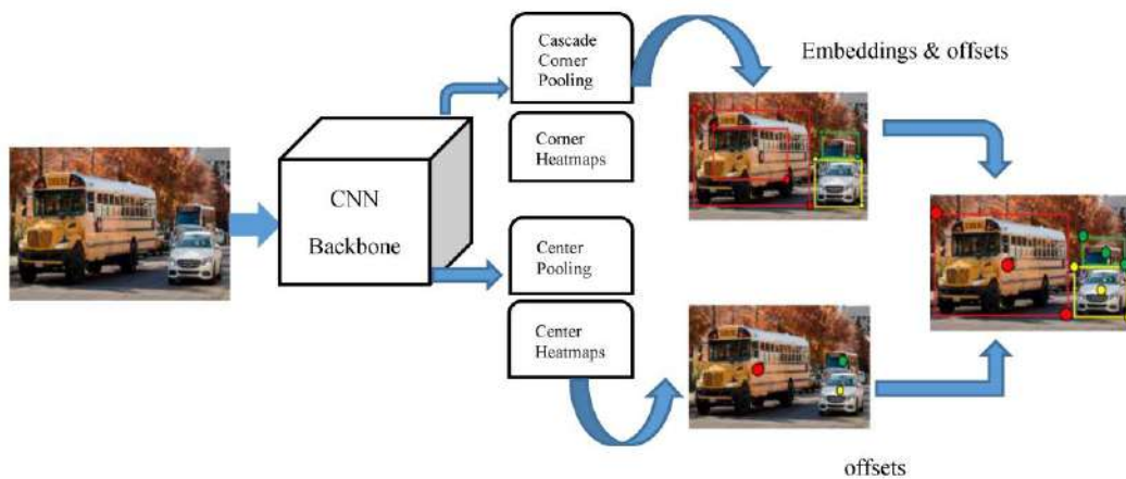
Figure 4. Architecture of CenterNet.
