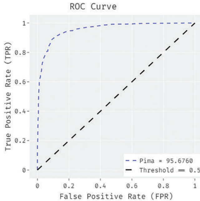
Figure 8: ROC analysis results of BDC-CMBOAI technique under Pima Indians diabetes dataset
