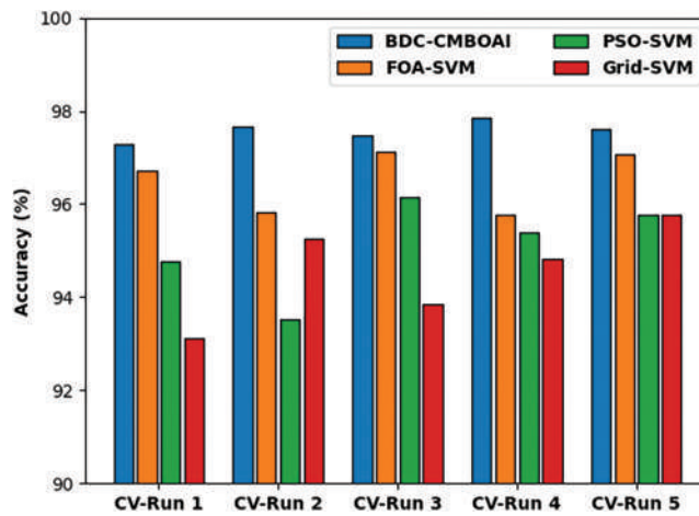
Figure 9: Accuracy analysis of BDC-CMBOAI technique under Thyroid dataset
