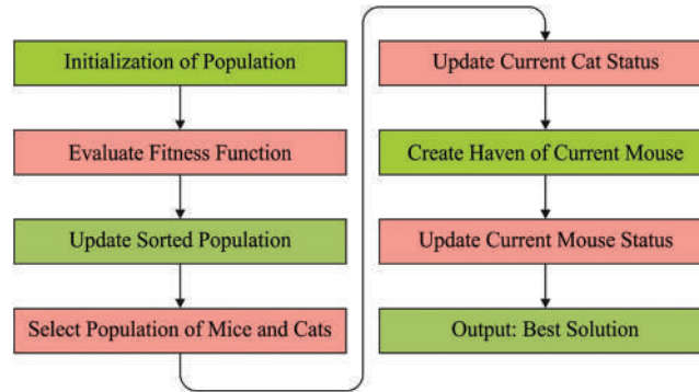
Figure 2: Process in CMO
