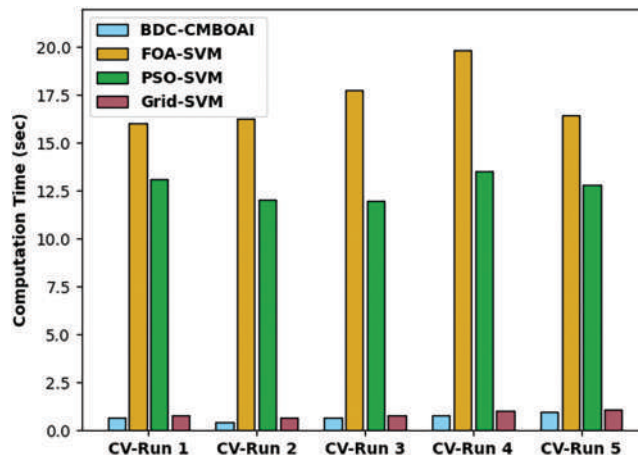
Figure 10: CT analysis of BDC-CMBOAI technique under Thyroid dataset
