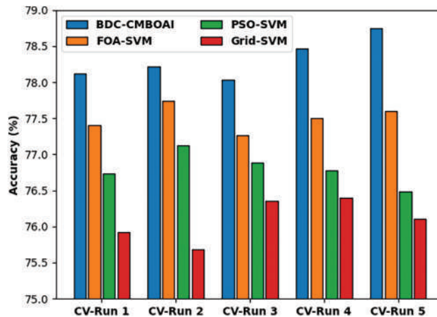
Figure 6: Accuracy analysis results of BDC-CMBOAI technique under Pima Indians diabetes dataset
