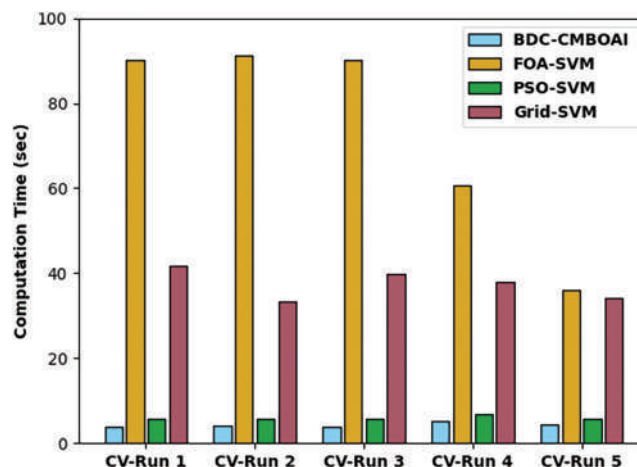
Figure 4: CT analysis of BDC-CMBOAI technique under Wisconsin breast cancer dataset
