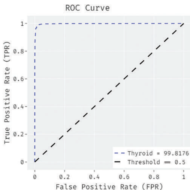
Figure 11: ROC analysis results of BDC-CMBOAI technique under Thyroid dataset
