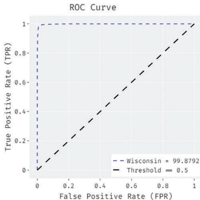
Figure 5: ROC analysis results of BDC-CMBOAI technique under Wisconsin breast cancer dataset
