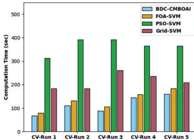
Figure 7: CT analysis of BDC-CMBOAI technique under Pima Indians diabetes dataset
