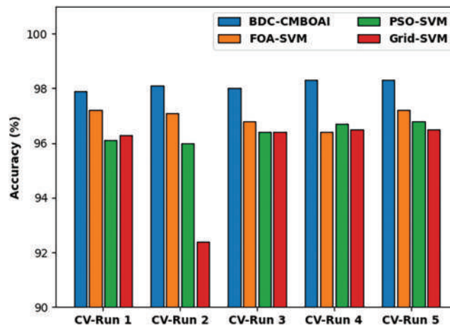
Figure 3: Accuracy analysis of BDC-CMBOAI technique under Wisconsin breast cancer dataset
