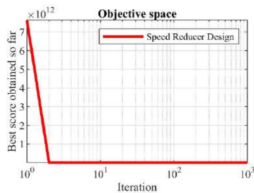
Figure 11. LOA’s performance convergence curve on speed reducer design.
