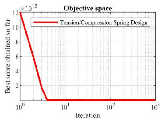
Figure 15. LOA's performance convergence curve on tension/compression spring.
