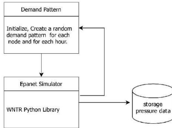
Figure 5. Flowchart of training data procedure.
