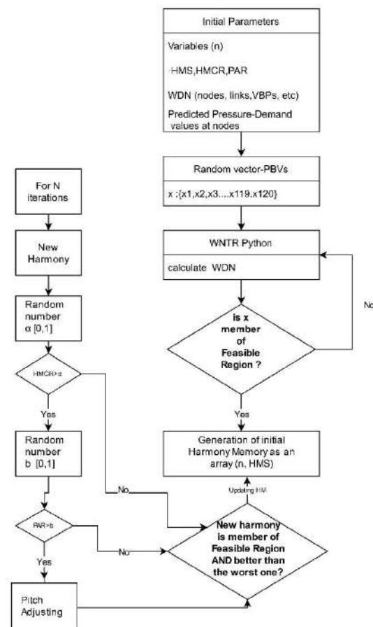
Figure 11. Flowchart of Harmony Search Algorithm.
